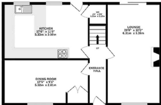
GROUND FLOOR 658 sq.ft. (61.1 sq.m.) approx.
